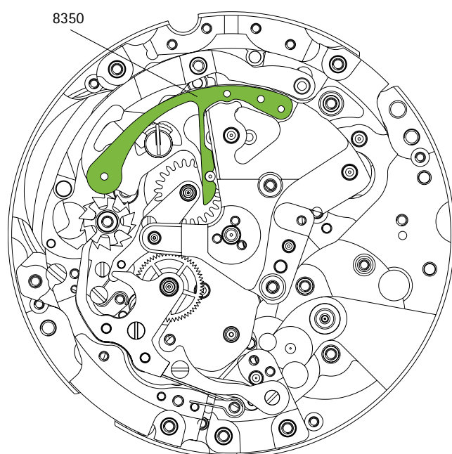
Hammer spring (8350)
