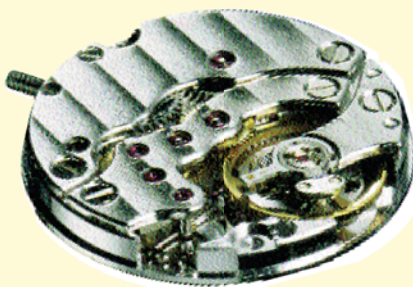
(6.10), Manual Wind, Ø 6 3/4 Ligne, Height 2.1mm, Jewels 21, Related Calibres: Calibre 615, See Entry
