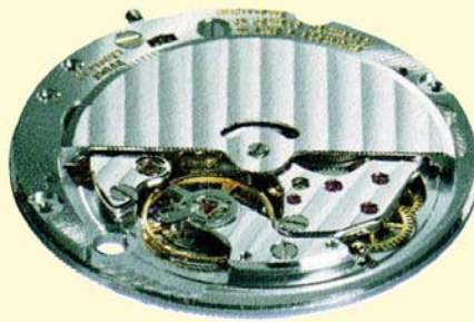
Automatic, Ø 12 Ligne, Height 2.4mm, Jewels 35, Related Calibres: Calibre 70 See Calibre 71 Entry, Calibre 716 Same as 71 with Sub Seconds 5h,
