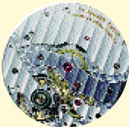
Manual Wind, Ø 15 3/4 Ligne, Height 1.9mm, Jewels 18, Related Calibres: Calibre 151, Same as 15 with Small seconds Calibre 152, Same as 15 with 24-Hour Hand
