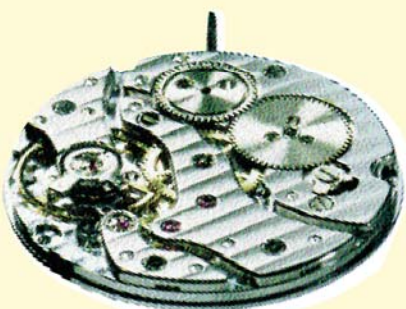
Manual Wind, Ø 9 Ligne, Height 1.73mm, Jewels 18, Related Calibres: Calibre 21P, Same as 21, Skeletonized.
