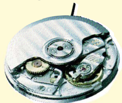
950 or 951 (9.51), Automatic, Seconds, Date Ø 9 Ligne, Height 3.25mm, Jewels 19, Related Calibres: Calibre 953, Same as 951 Without Date, Calibre 9511, Same as 951 with Ø10 1/2 Ligne, Calibre 9531, Same as 951 with Ø10 1/2 Ligne, Date Calibre 9516, Same as 951 with Ø10 1/2 Ligne, 24-Hour Hand.
